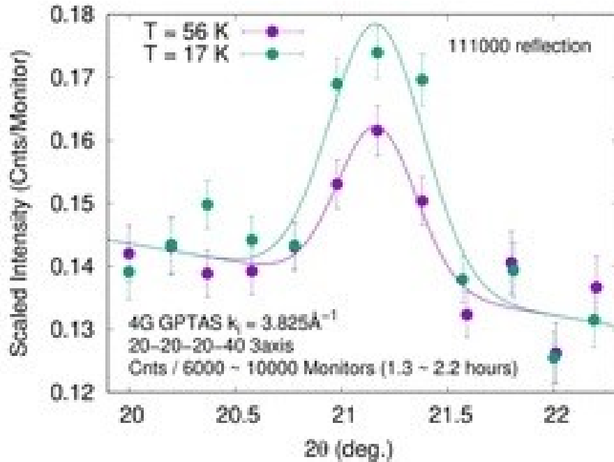
The peak profile around the 111000 reflection in the icosahedral \text{Al}_{65}\text{Ga}_{20}\text{Gd}_{15} QC at temperatures below and above the Curie temperature [13].
