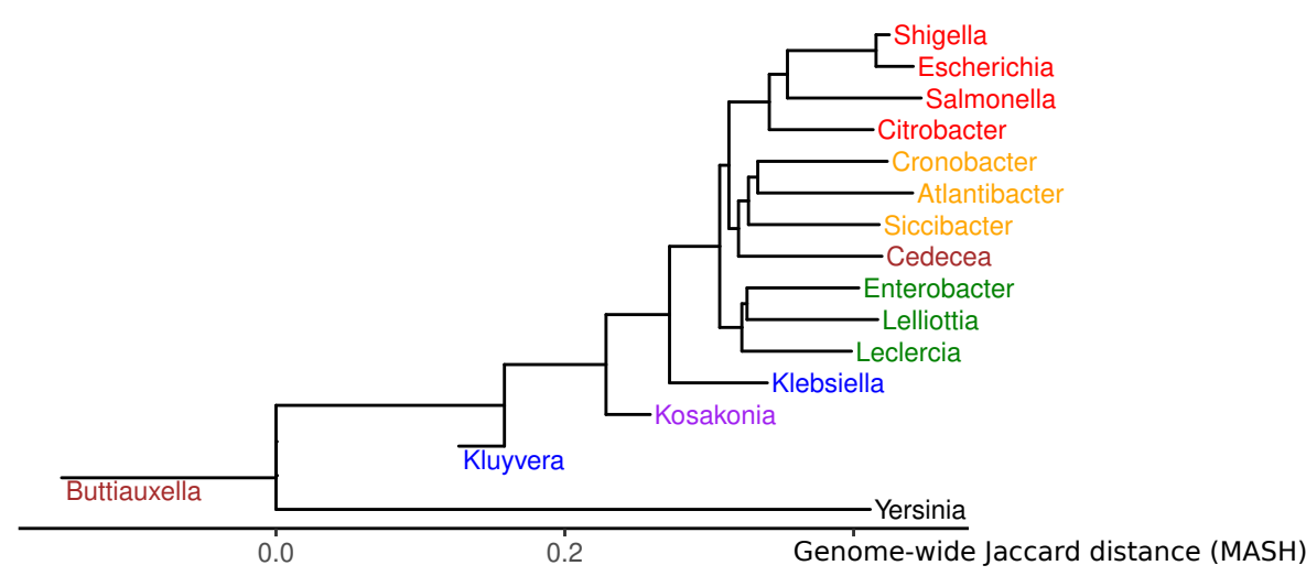
MASH NJ Tree with Colored Clades
