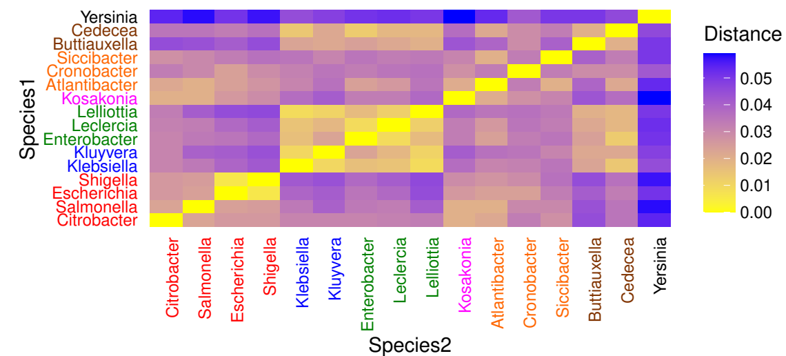
ANI Heatmap with Clade Colors
