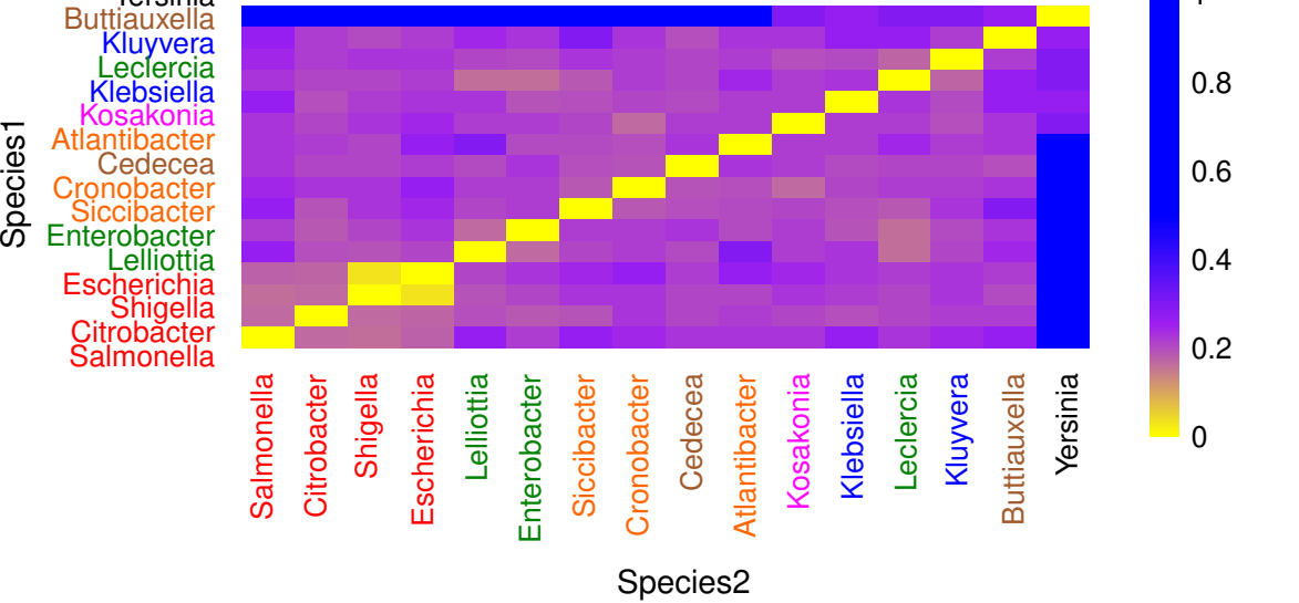
MASH Distance Heatmap with Clade Colors
