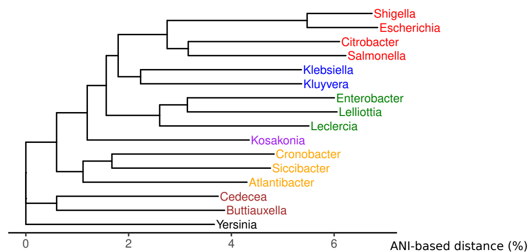
MASH NJ Tree with Colored Clades
