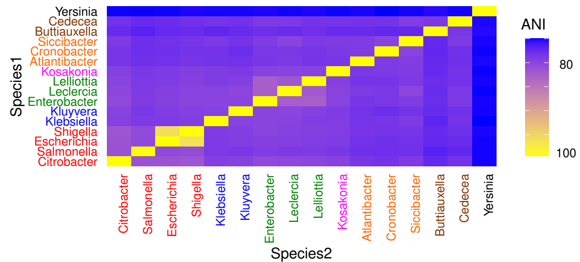
MASH Distance Heatmap with Clade Colors
